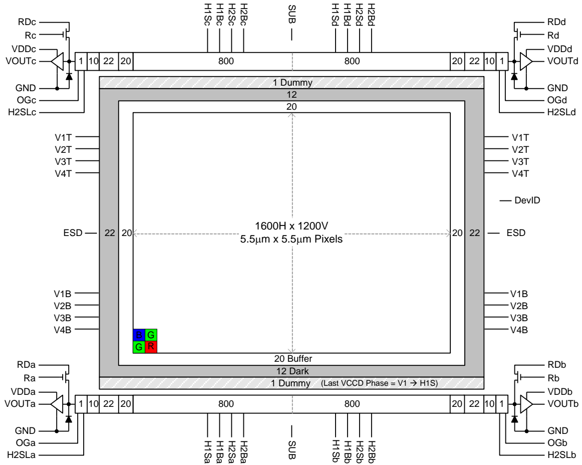
Figure 1: Block Diagram
