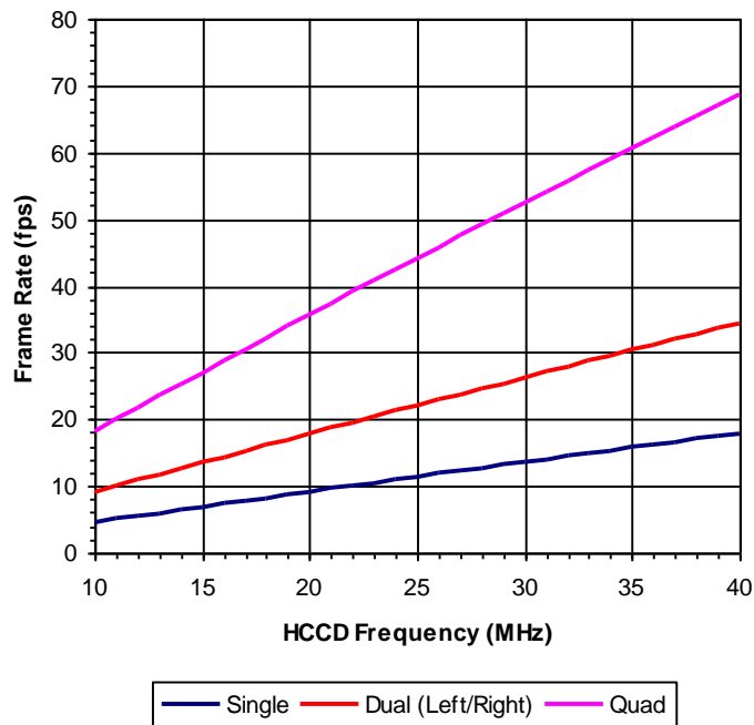
Figure 11: Frame Rates
